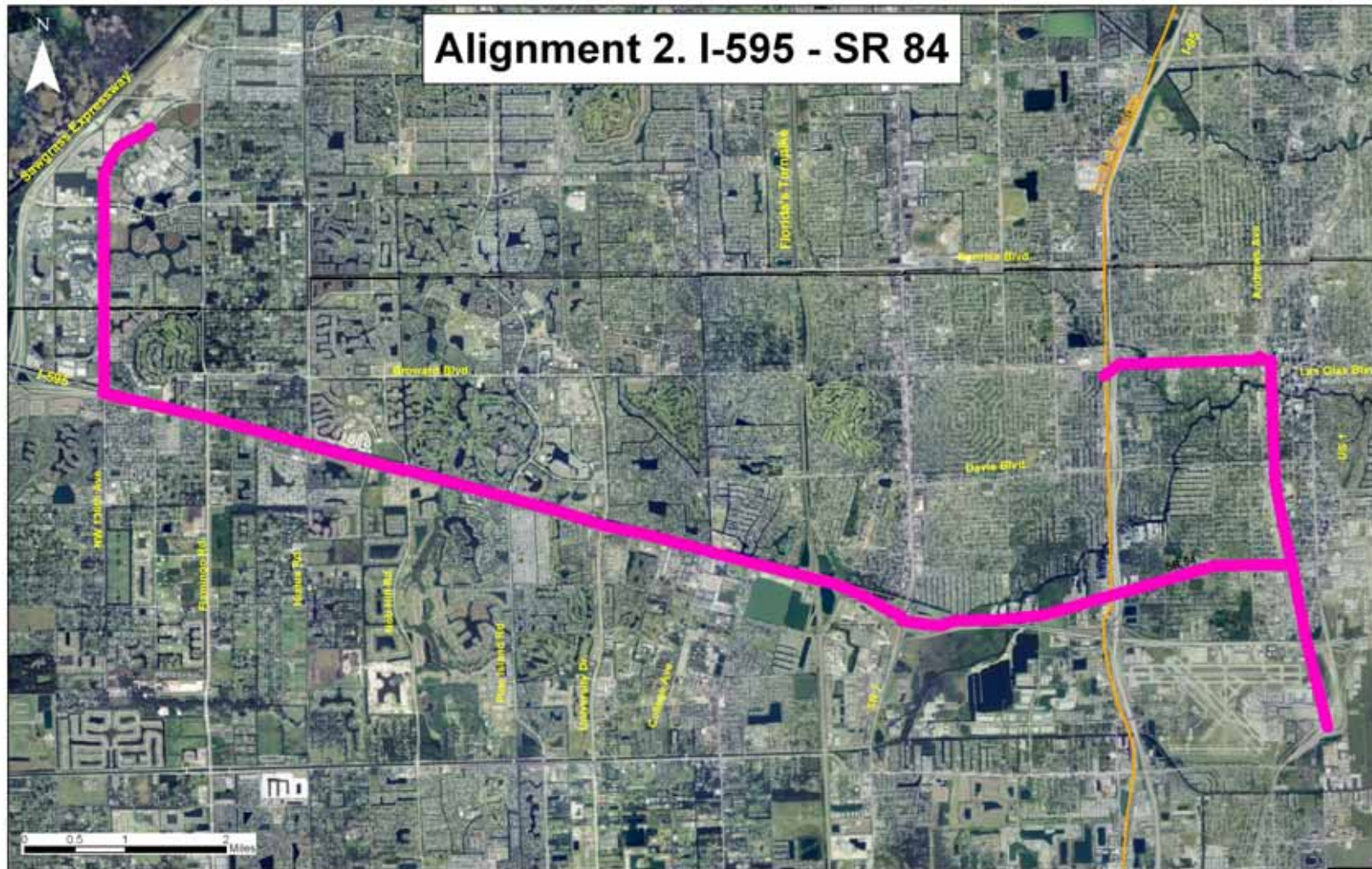
Figure 4: Alignment 2 (I-595/SR 84/Andrews Avenue)
