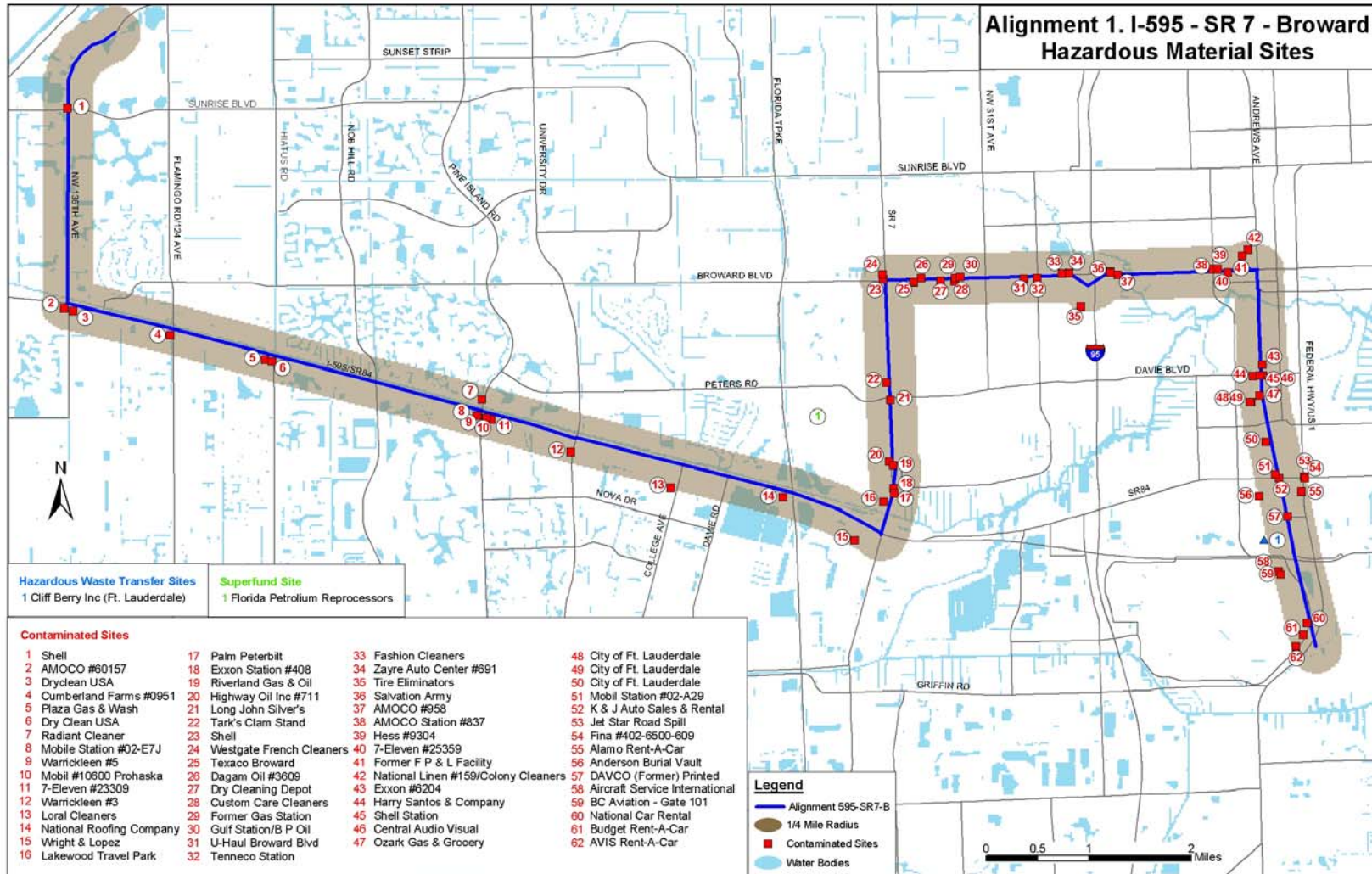
Figure 8: Potential Hazardous Materials Sites along Alignment 1
